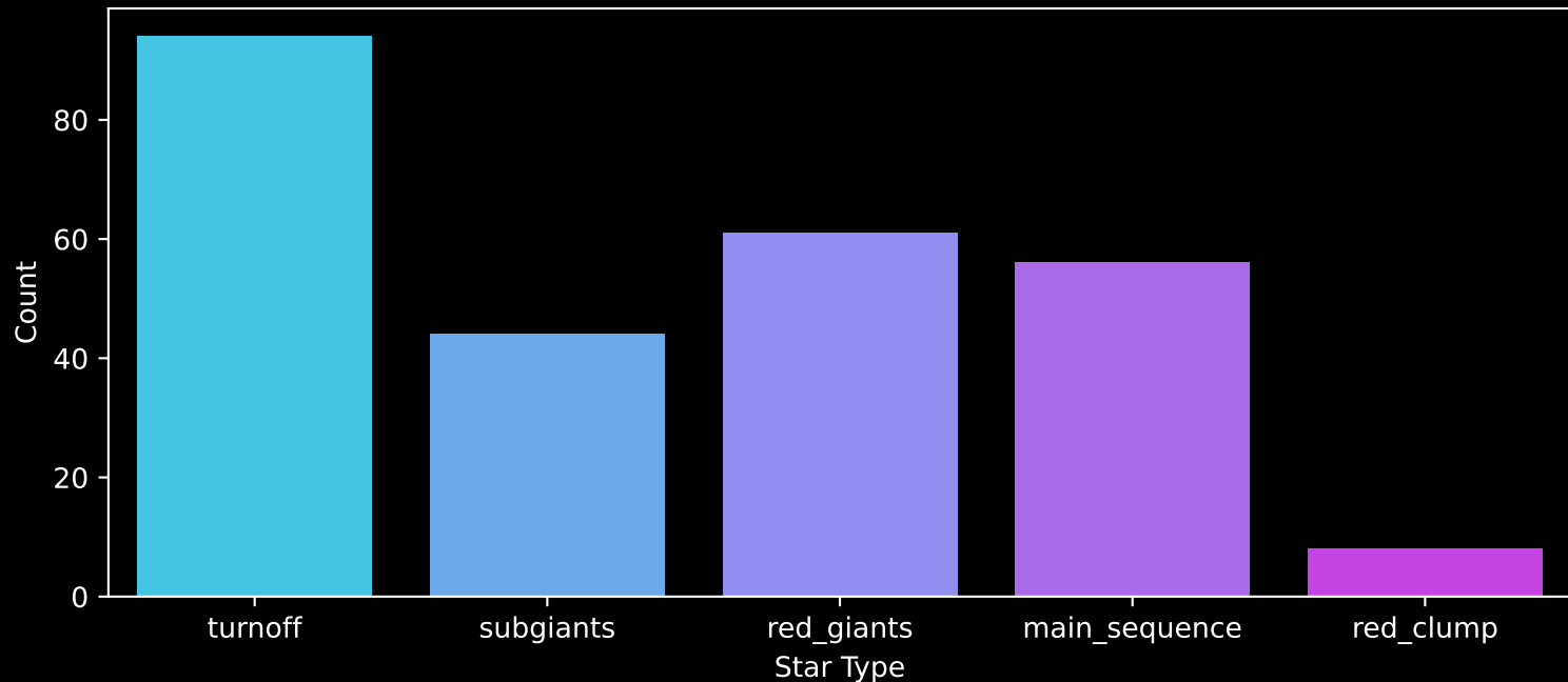
GALAH DR4 Field: [9397] Count plot of Star Type
