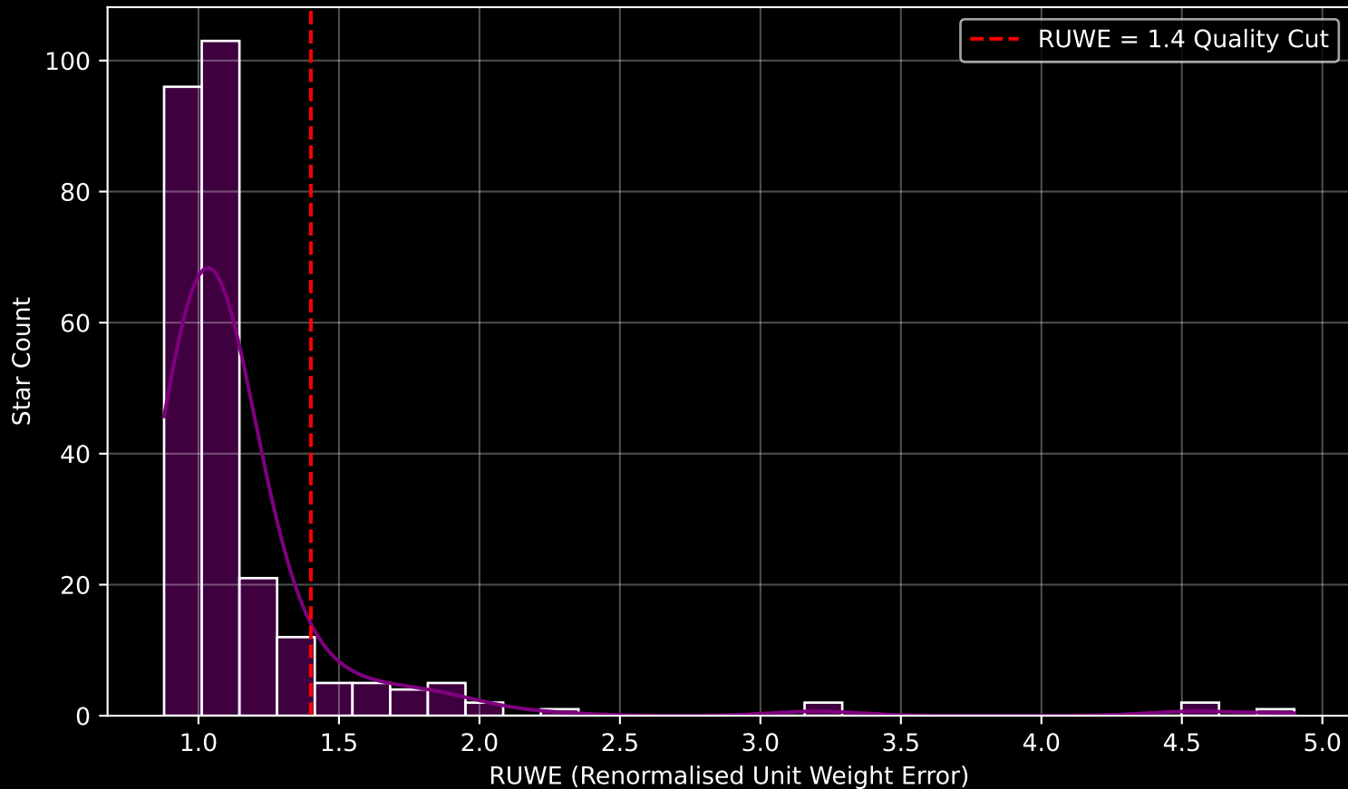
GALAH DR4 Field [9397] RUWE Distribution (n= 259)
