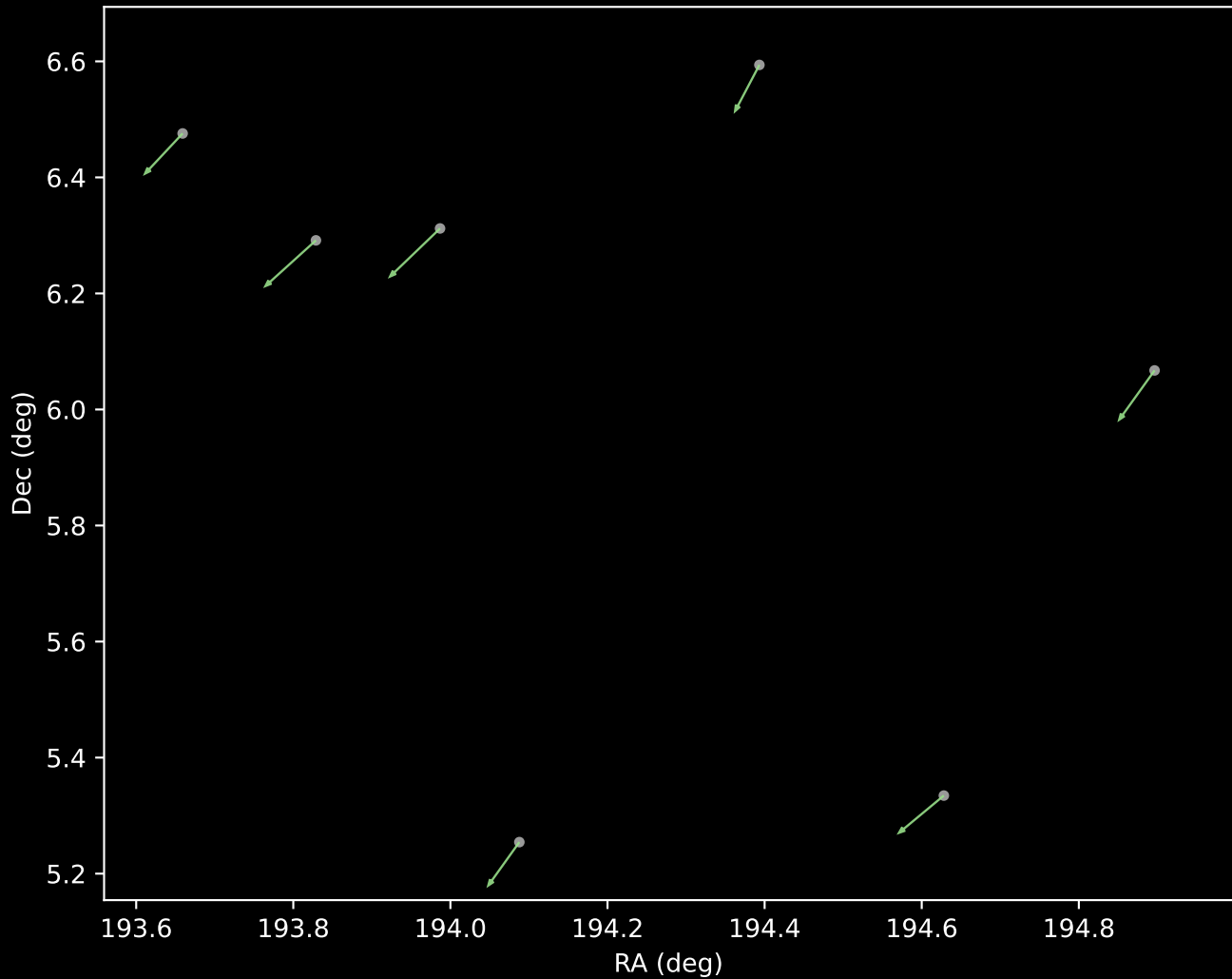
GALAH DR4 Cluster 5 Proper Motion Vectors (n=7)
