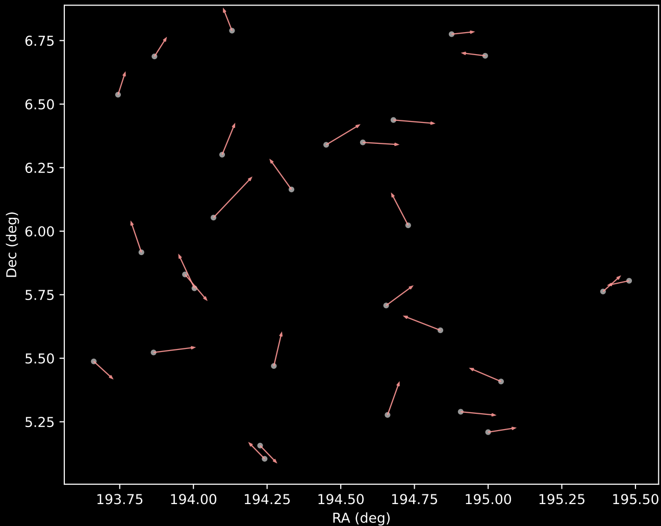
GALAH DR4 Cluster 7 Proper Motion Vectors (n=28)
