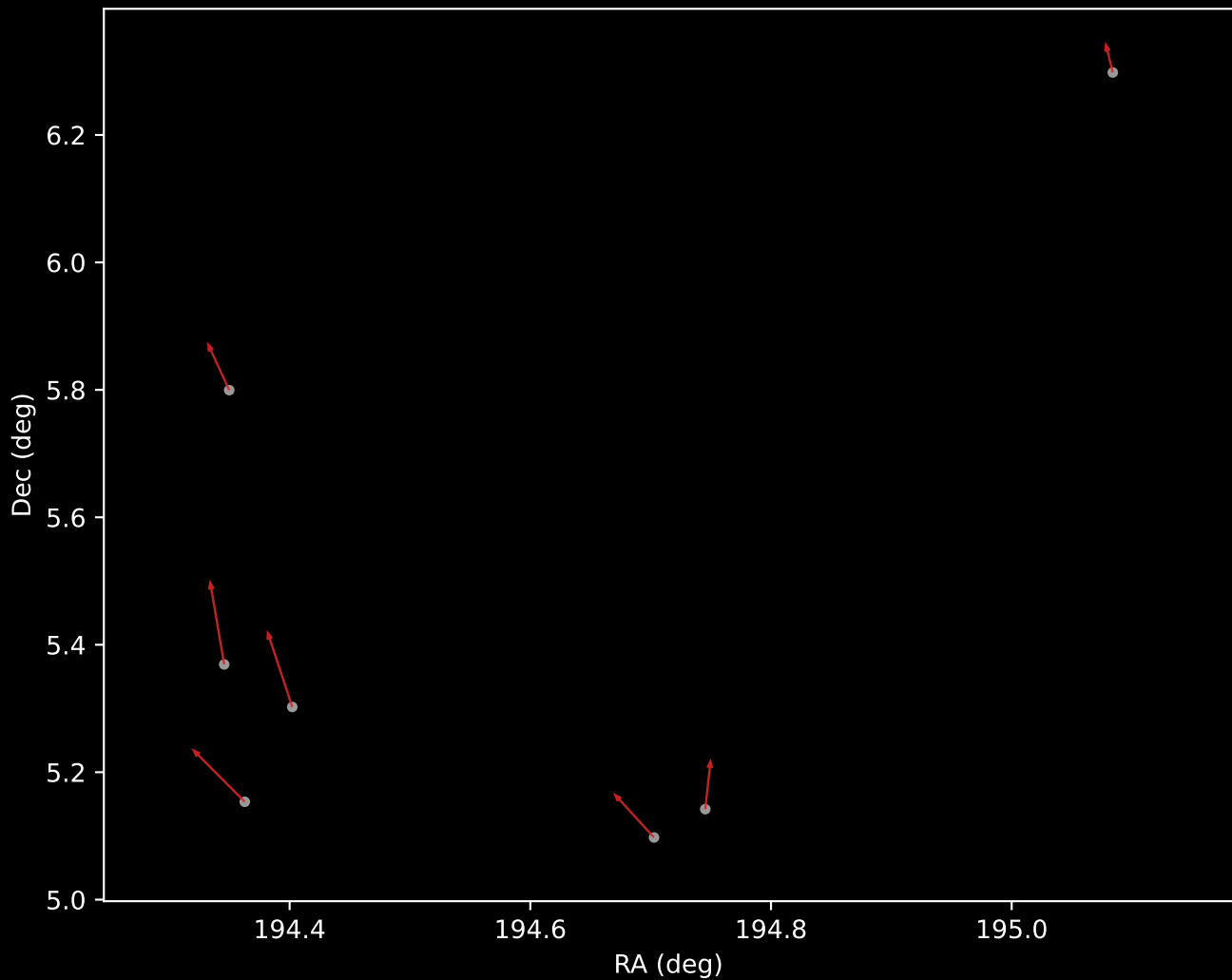
GALAH DR4 Cluster 6 Proper Motion Vectors (n=7)
