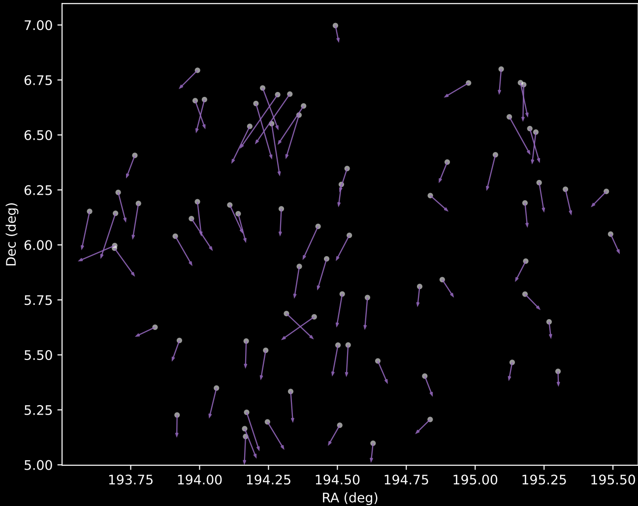
GALAH DR4 Cluster 8 Proper Motion Vectors (n=75)
